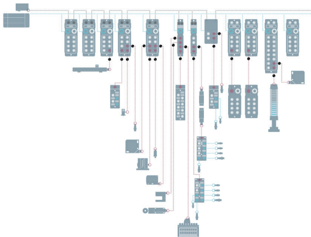
Networking PLCs and IO-Link masters (various fieldbuses) and connecting to IO-Link field devices in a machine
